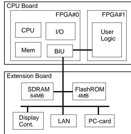
Figure 6: Mappi: the M32R FPGA evaluation board; it has the M32R softmacro on FPGA (CPU, MMU, Cache, SDI, SDRAMC, UART, Timer), FPGA Xilinx XCV2000E \times 2 , SDRAM(64MB), FlashROM, 10BaseT Ethernet, Serial 2ch, PC-card slot \times 2 , and Display I/F(VGA)
