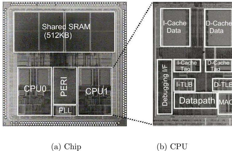
Figure 5: A micrograph of an on-chip-multiprocessor M32R prototype chip
