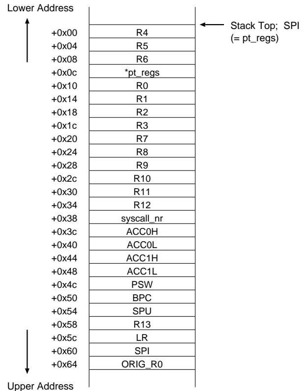
Figure 3: Stack frame formed by a system call
